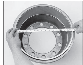
1. Braking surface diameter
